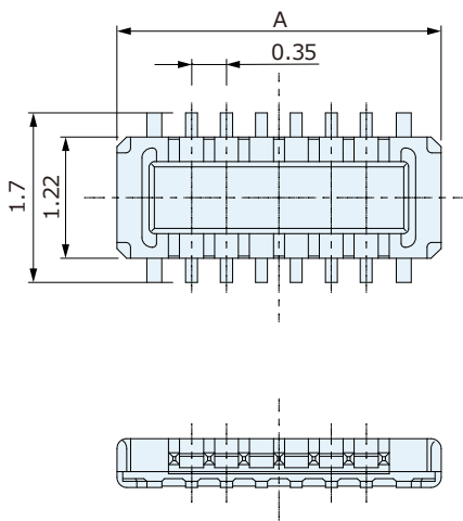
Plug : CPBE8□□-0101F
