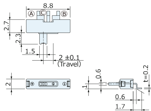
Outline Drawing : SMT Terminal JSB1220-1821F
