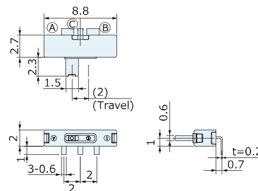
Outline Drawing : Discrete Terminal JSB1220-1721F
