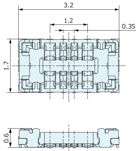
插头：CPBD408-0101F
